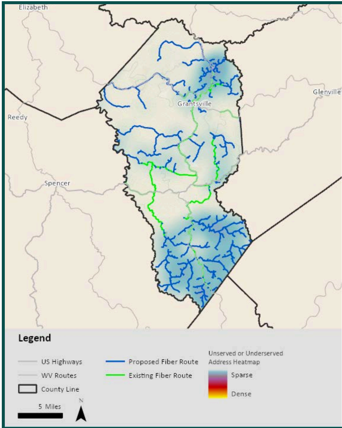
Figure 18. Current and Proposed Fiber Routes and address clusters, Calhoun County
