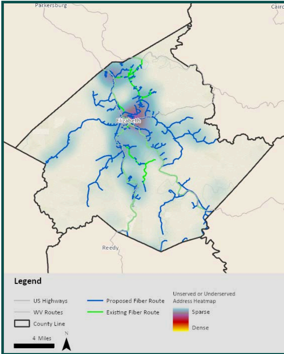
Figure 19. Current and Proposed Fiber Routes and address clusters, Wirt County
